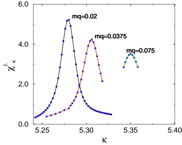
Fig. 3. The Polyakov loop temperature susceptibility \chi_{\kappa}^K as function of the temperature variable \kappa = 6/g^2
