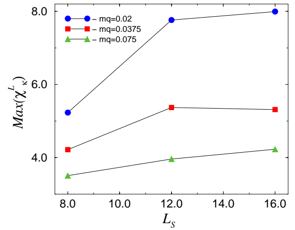
Fig. 6. The dependence of the \chi_{\kappa}^L peak height on spatial lattice size
