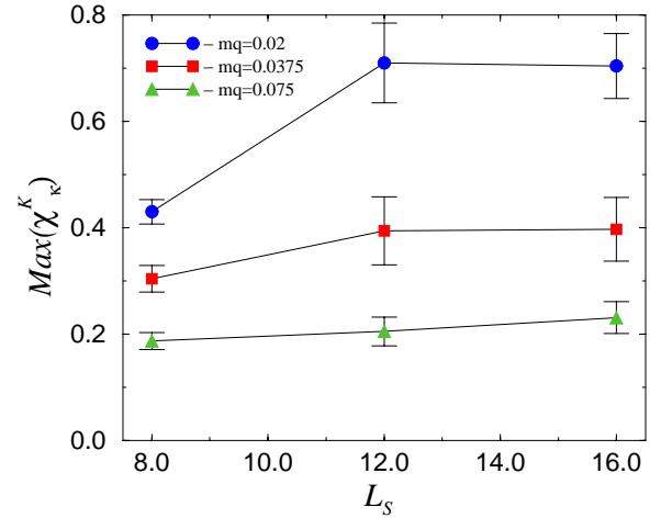
Fig. 5. The dependence of the \chi_{\kappa}^K peak height on spatial lattice size
