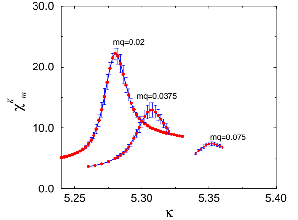
Fig. 2. The chiral quark mass susceptibility \chi_m^K as function of the temperature variable \kappa = 6/g^2
