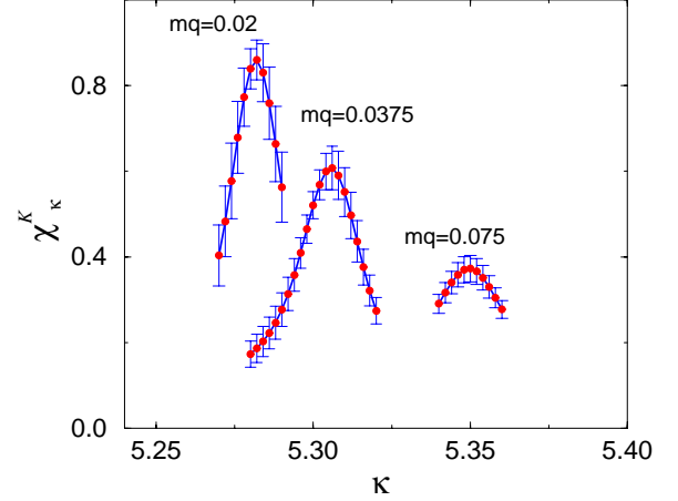
Fig. 1. The chiral temperature susceptibility \chi_\kappa^K as function of the temperature variable \kappa = 6/g^2
